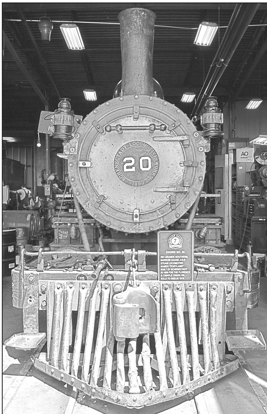
RGS No. 20 in the CRRM roundhouse on July 10, 2019, for the completion of the restoration. – Photo © 2019 Bruce Nall.
